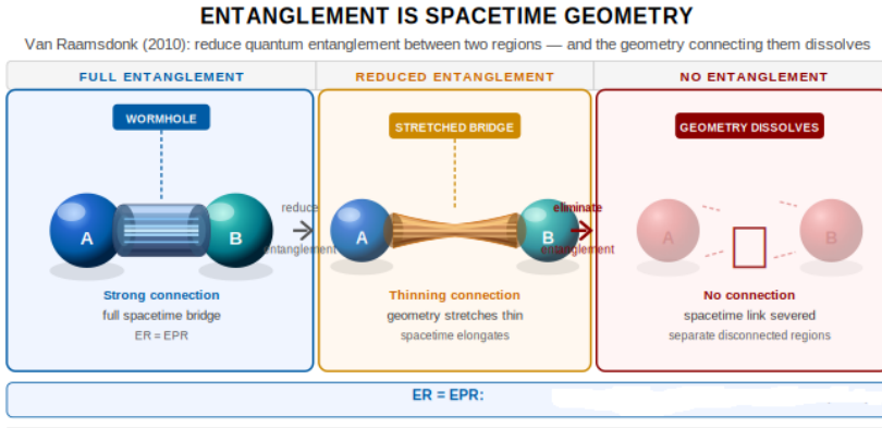
Figure 15 - 1 Van Raamsdonk (2010): "Building up spacetime with quantum entanglement." The degree of entanglement between boundary regions corresponds precisely to geometric connectivity in the bulk spacetime.
